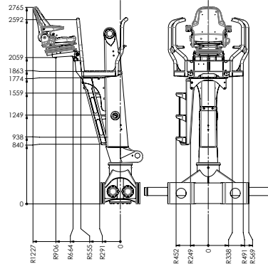
High pillar
